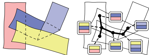
Figure 8: List graph.
