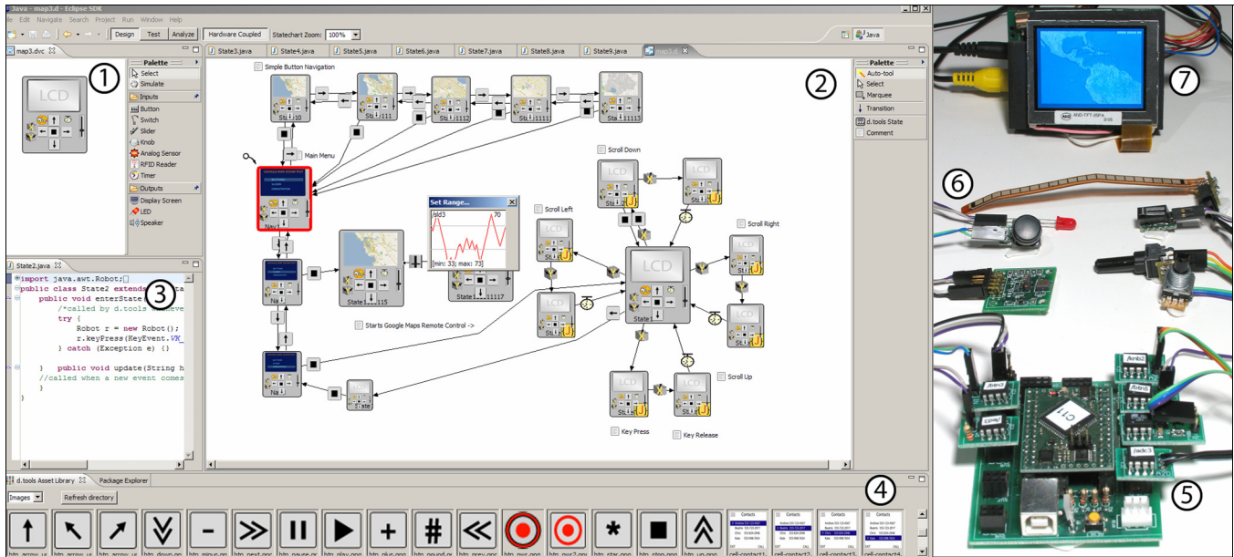
Figure 2 Left: The d.tools authoring environment offers (1) a device designer; (2) a statechart editor; (3) a source code editor; and (4) an image browser. Right: The d.tools hardware interface (5) connects compatible hardware inputs (6) to the PC. d.tools includes authoring support for small LCD screens (7).
